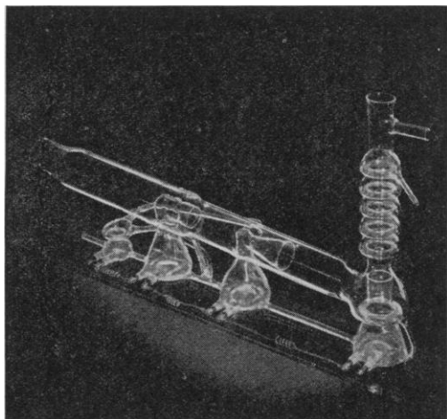
Glass Three-stage Fractionating Pump, Type GF-25A (air-cooled)
