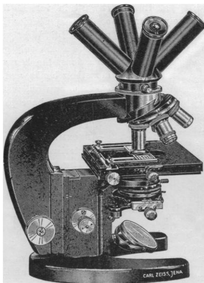
A new universal stable stand
