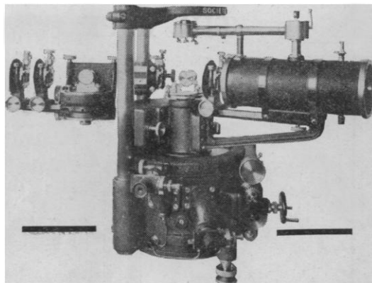
The Compton Spectrometer
