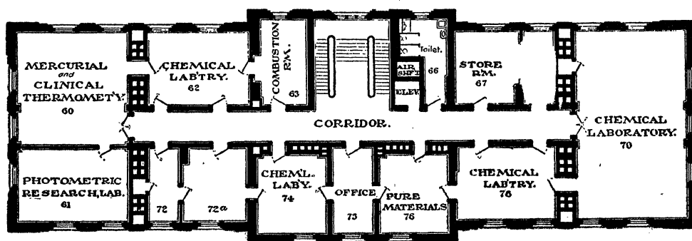
4th.FLOOR PLAN.
