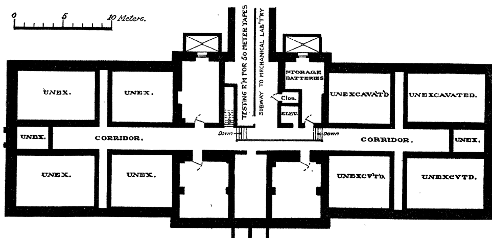
BASEMENT PLAN.
