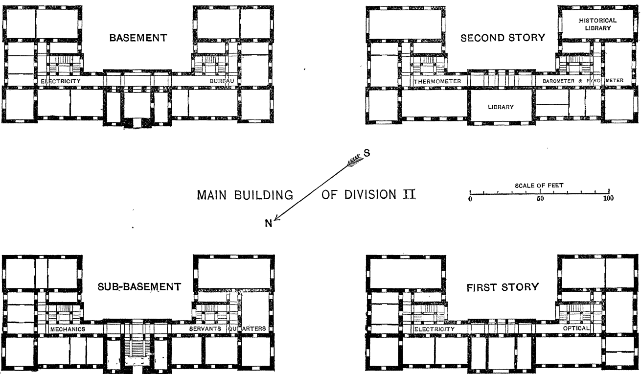
FIG. 2.—Floor Plans of Main Building. Division II.
