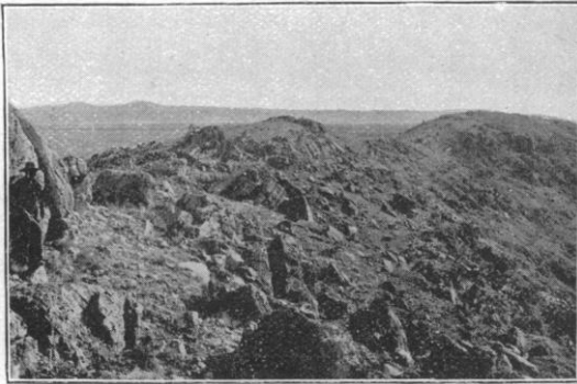
FIG. 1.—Rim of Coon Butte, with part of inner face.
