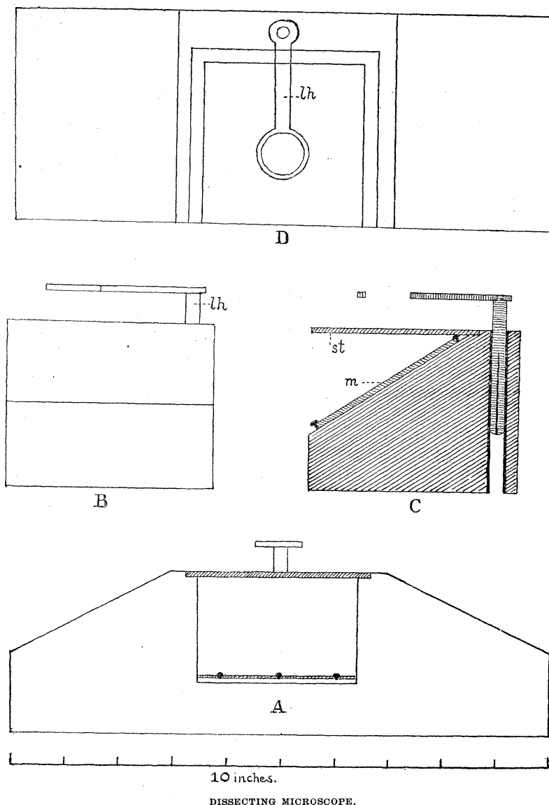
DISSECTING MICROSCOPE. The body is a solid block of clear pine, cut as shown in A , front view; B , end view; C , median cross section; D , top view. lh , lens holder, which slides in brass tube driven into a hole in block (sec. C .); st , stage, a movable glass plate; m , mirror, fastened with small screws or tacks.
