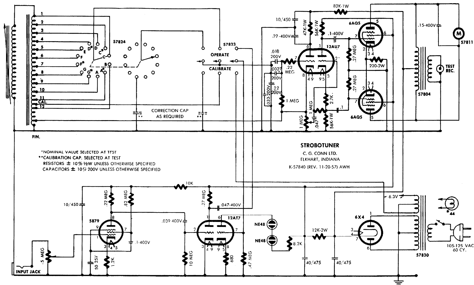
Figure 5—Strobotuner, Model ST-2, Schematic Diagram
