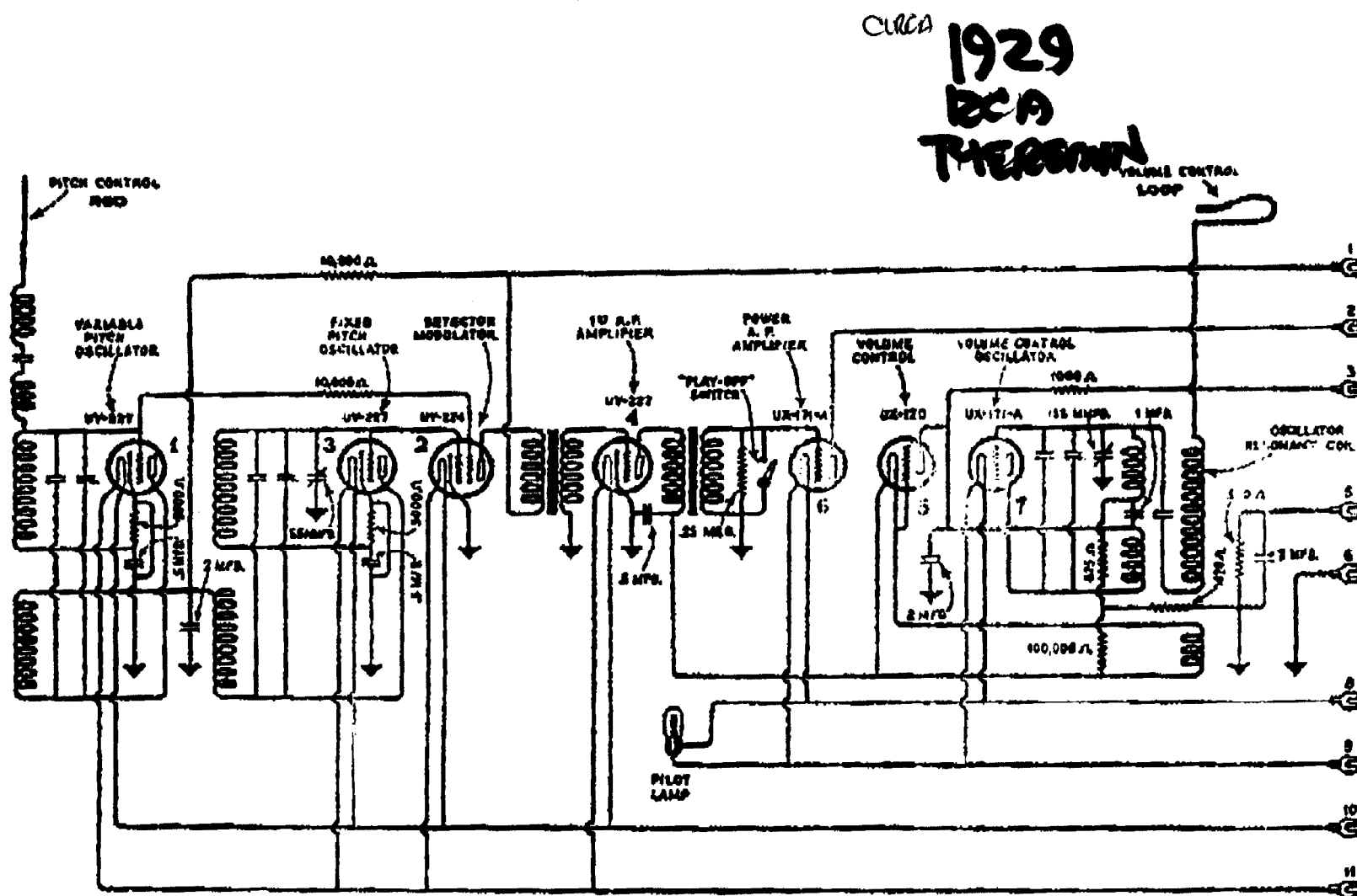
Figure 4—Schematic circuit diagram of the main assembly
