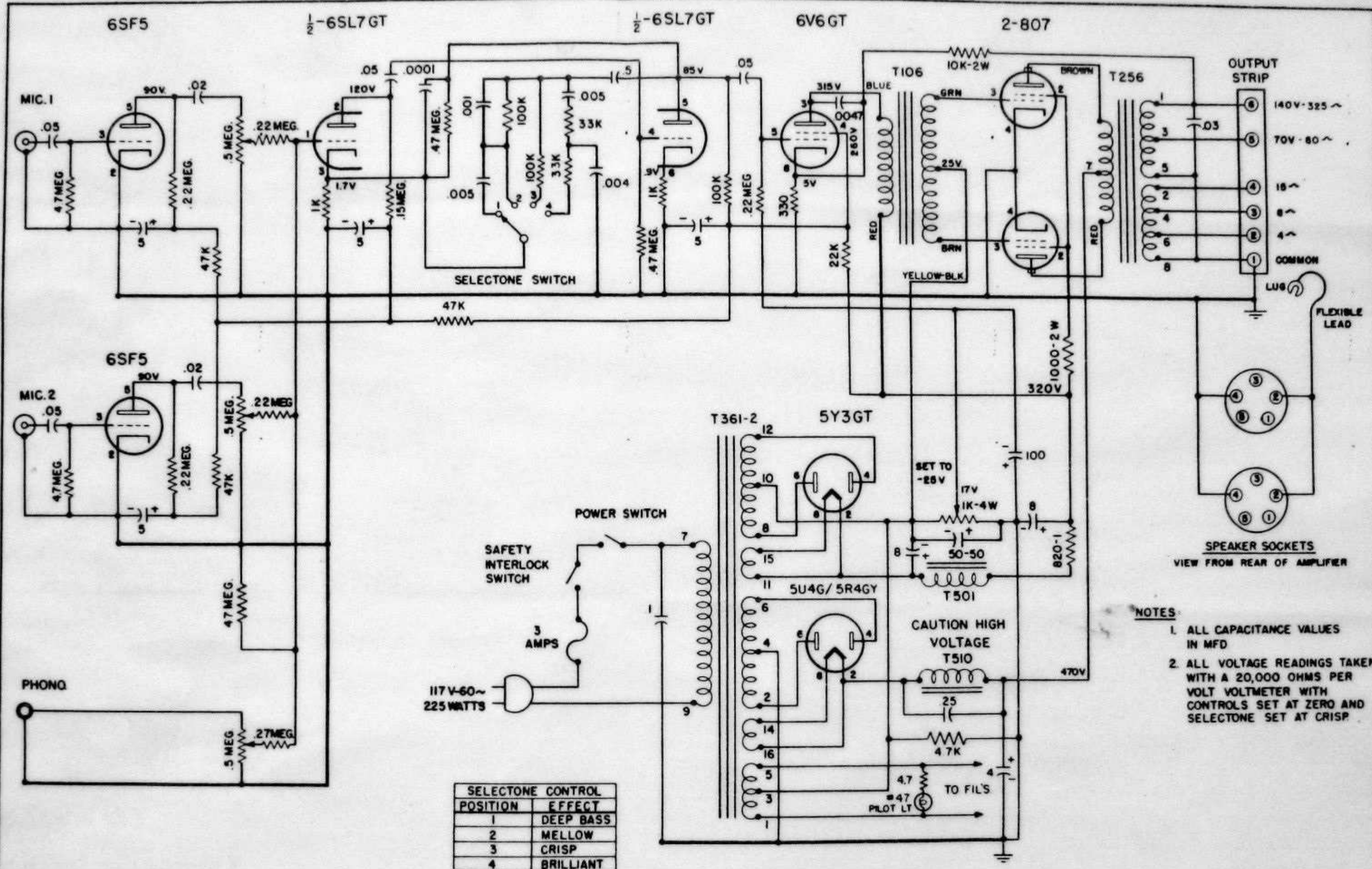
CHALLENGER MODEL CH60 Schematic Diagram Courtesy of Lear Siegler, Inc., Bogen Communications Div.
