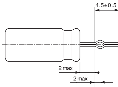
5 \leq \varnothing D \leq 8 Leads bent open, shortened and formed EKS 09... (S = 5 mm)
