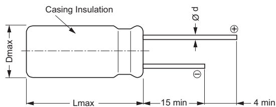
5 \leq \varnothing D \leq 18 Long leads EKS 00...
