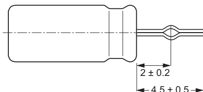
10 \leq \varnothing D \leq 18 Leads shortened and formed EKS 06... (S = 5 / 7.5 mm)
