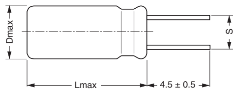
5 \leq \varnothing D \leq 18 Shortened leads EKS 05... (S = 2 / 2.5 / 3.5 / 5 / 7.5 mm)
