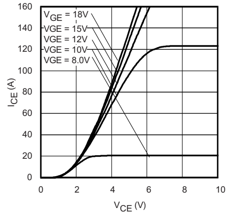
Fig. 5 - Typical IGBT Output Characteristics T_J = -40^\circ\text{C} ; t_p = 80\text{ }\mu\text{s}
