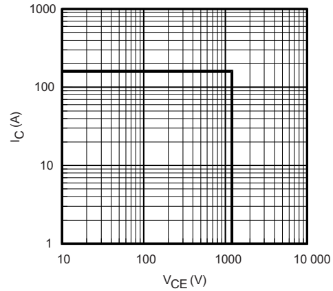
Fig. 4 - Reverse BIAS SOA T_J = 150^\circ\text{C} ; V_{GE} = 15\text{ V}
