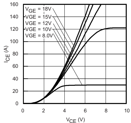
Fig. 6 - Typical IGBT Output Characteristics T_J = 25^\circ\text{C} ; t_p = 80\text{ }\mu\text{s}
