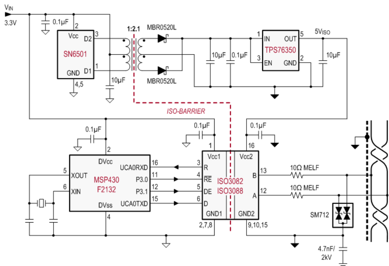
Figure 50. Isolated RS-485 Interface
