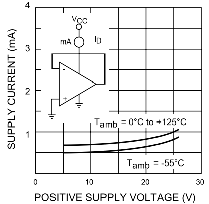
Figure 13: Supply current
