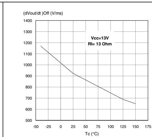
Figure 28. Turn-Off voltage slope
