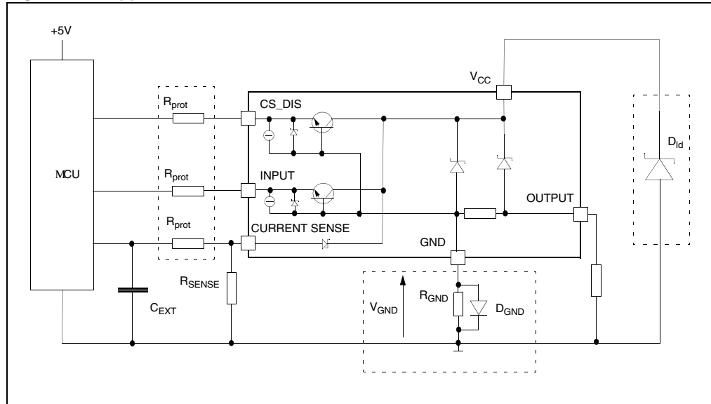
Figure 32. Application schematic
