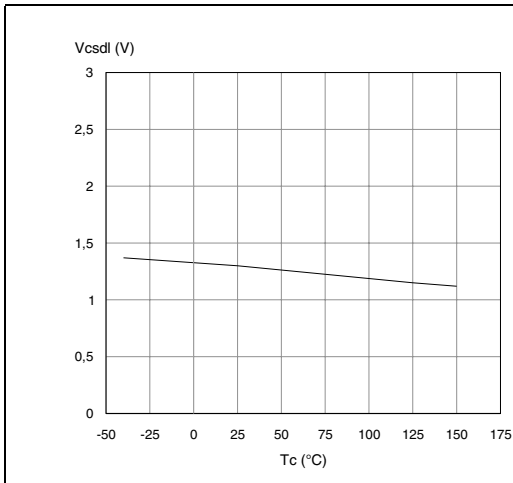
Figure 31. CS_DIS low level voltage
