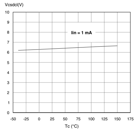
Figure 30. CS_DIS clamp voltage
