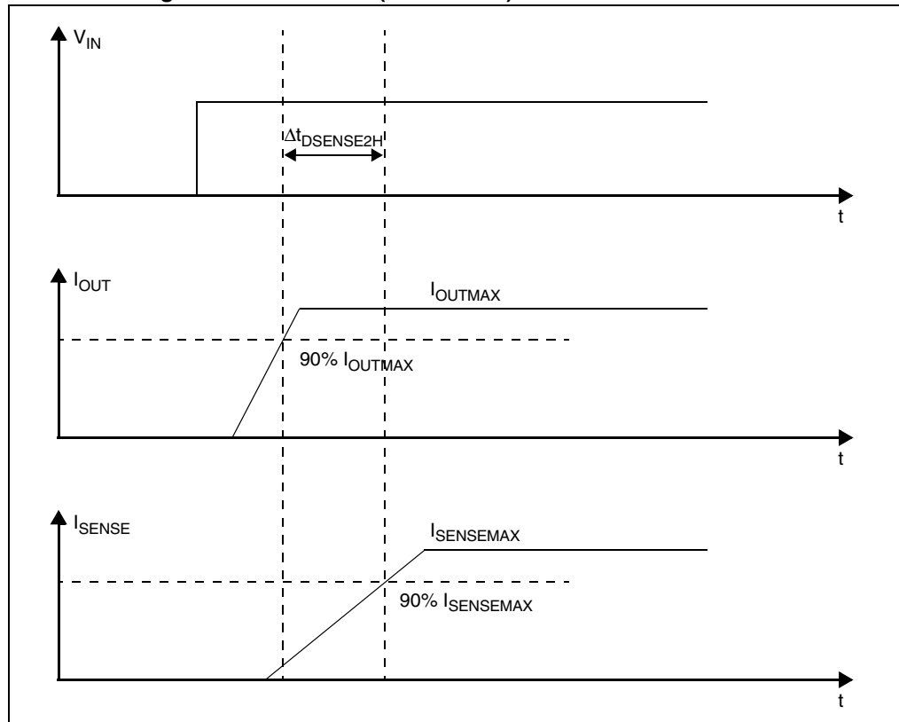
Figure 6. Switching characteristics
