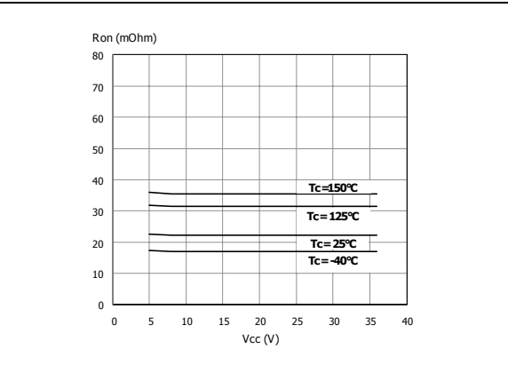
Figure 18. On state resistance vs V_{CC}
