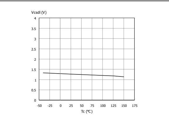
Figure 24. CS_DIS low level voltage
