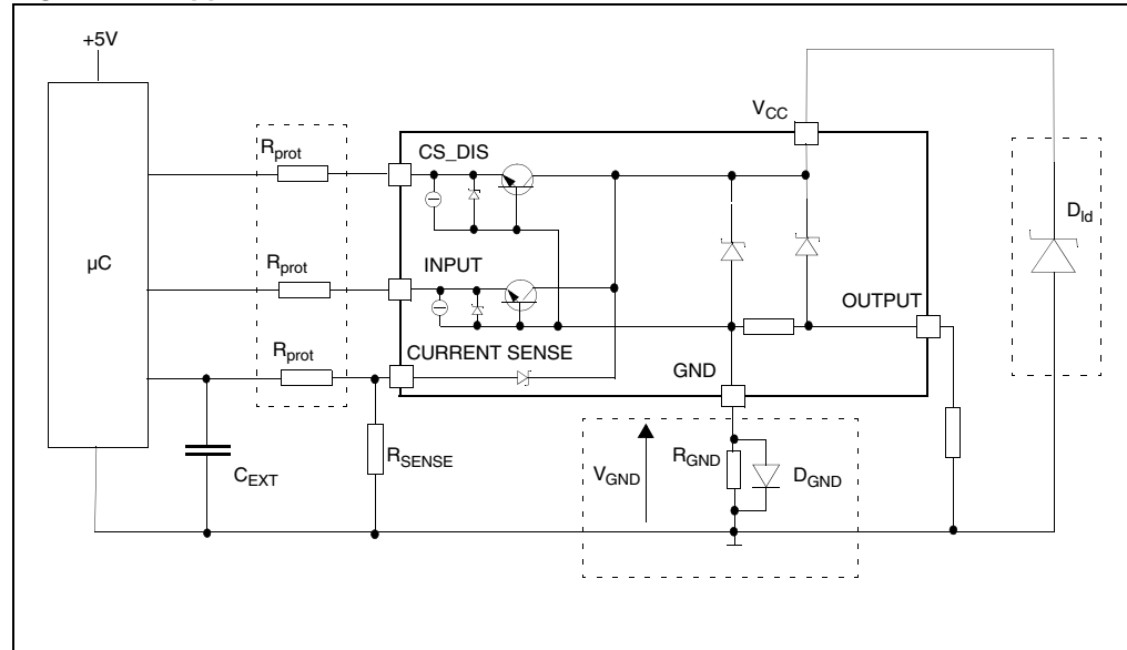
Figure 26. Application schematic
