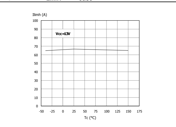
Figure 20. I_{LIMH} vs T_{case}
