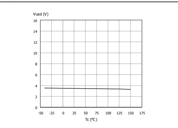
Figure 19. Undervoltage shutdown
