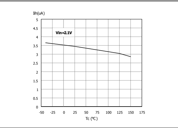
Figure 14. Input high level
