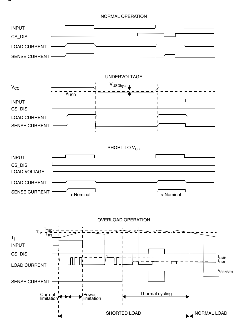
Figure 10. Waveforms
