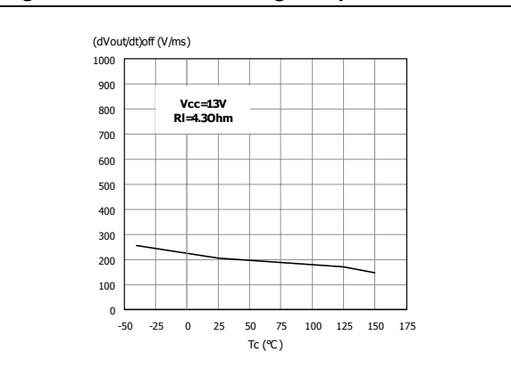
Figure 22. Turn-Off voltage slope
