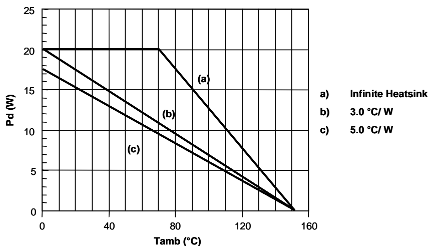
Figure 10. Power derating curve
