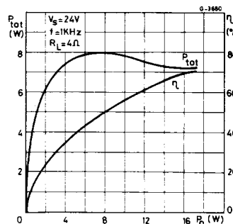
Figure 17. Power dissipation and efficiency vs. output power
