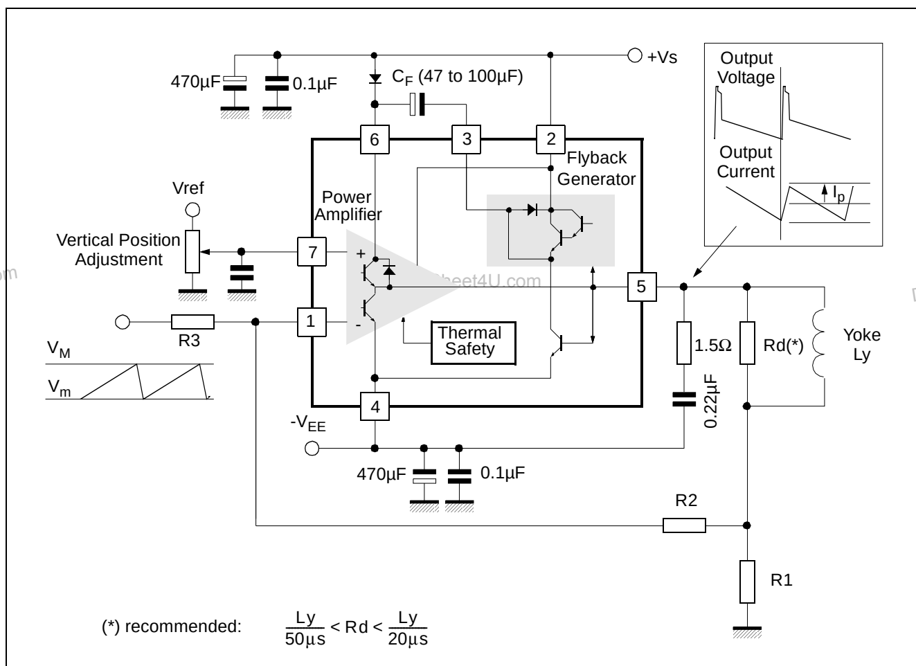
Figure 4: DC-coupled Application
