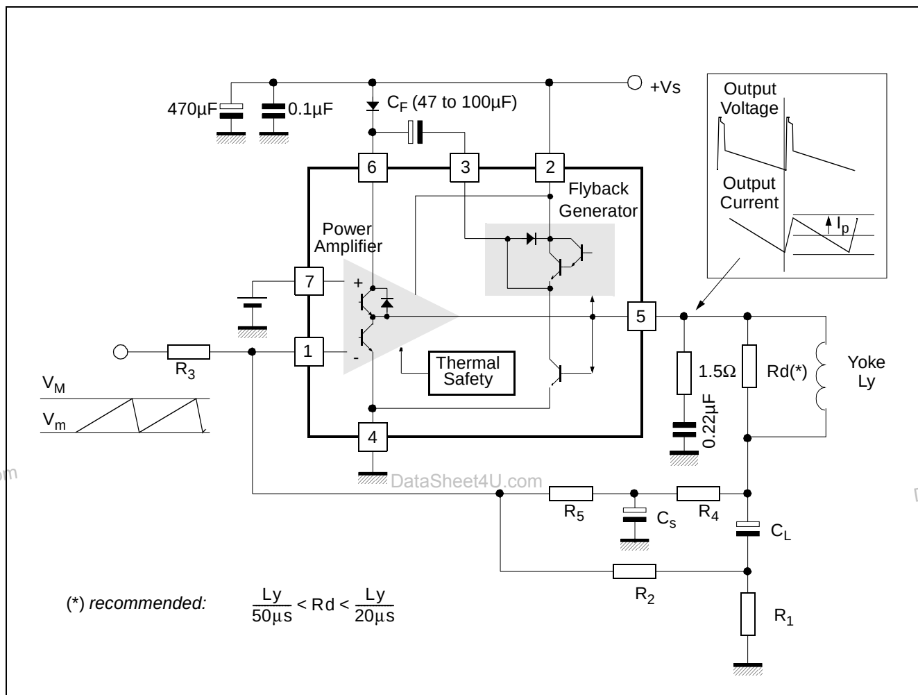
Figure 6: AC-coupled Application
