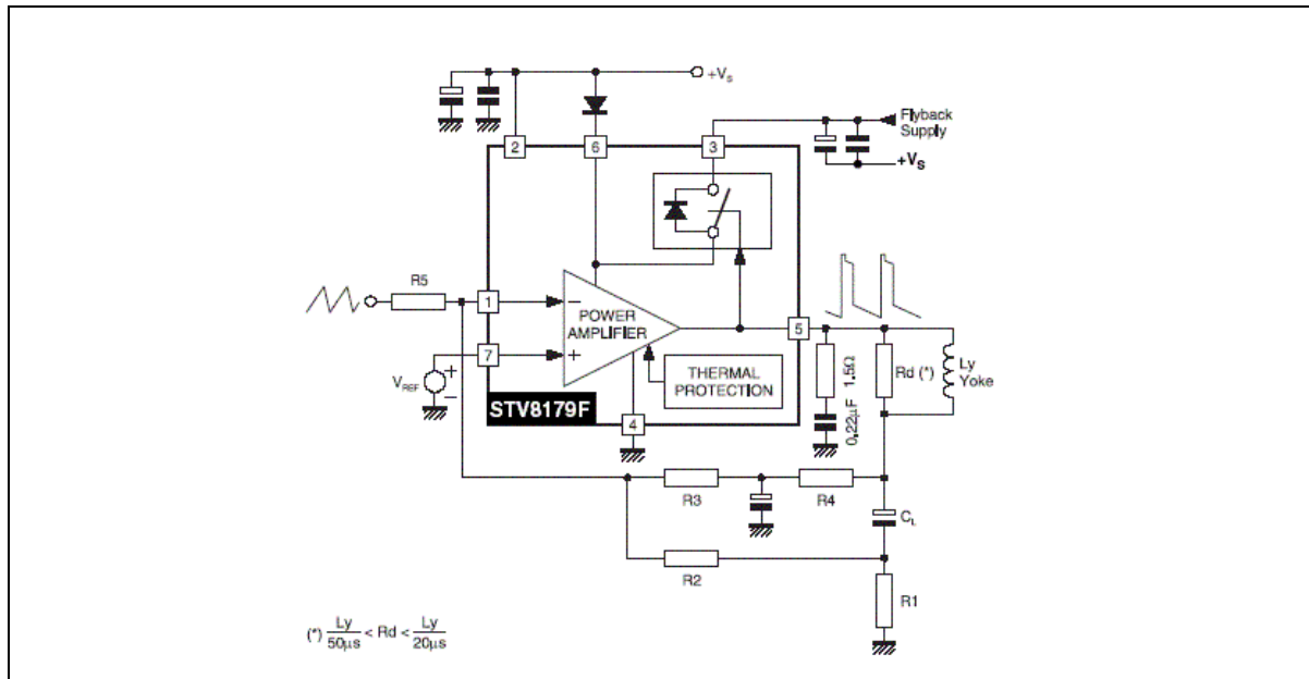
Figure 1: AC Coupling
