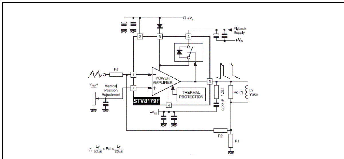
Figure 2: DC Coupling
