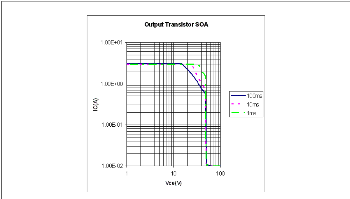
Figure 3: Output Transistor SOA (for Secondary Breakdown)
