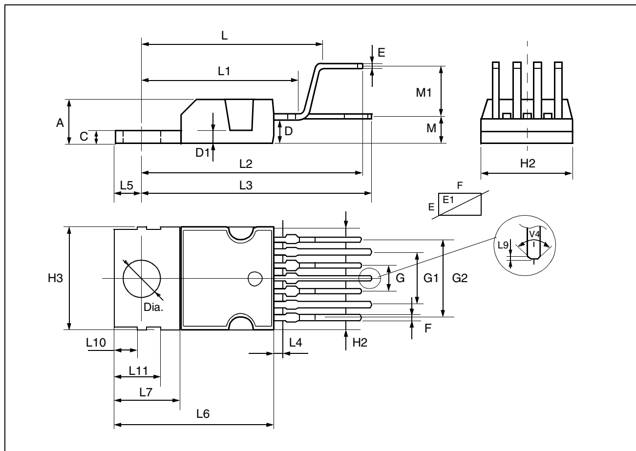
Figure 5: 7-pin Plastic Heptawatt Package
