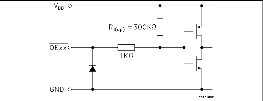
Figure 3. \overline{\text{OE}}_{\text{xx}} terminal
