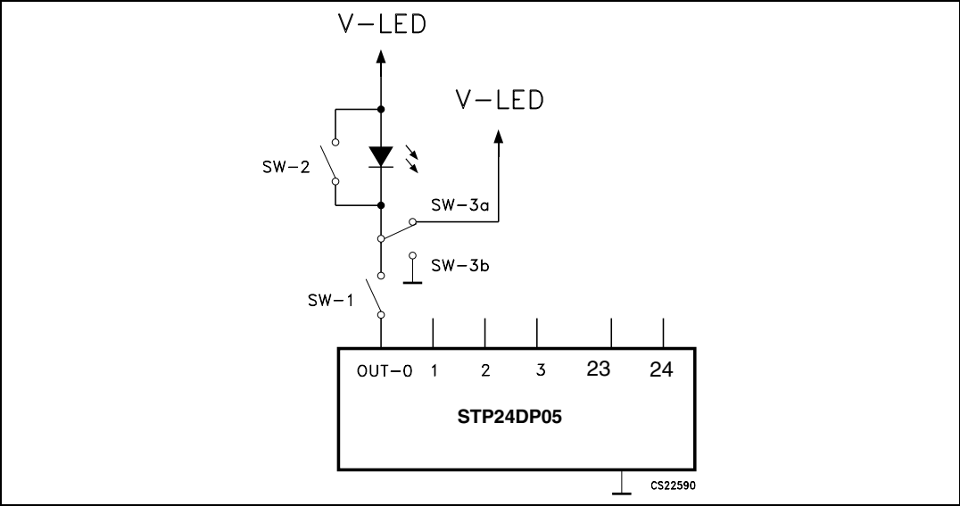
Figure 12. Detection circuit
