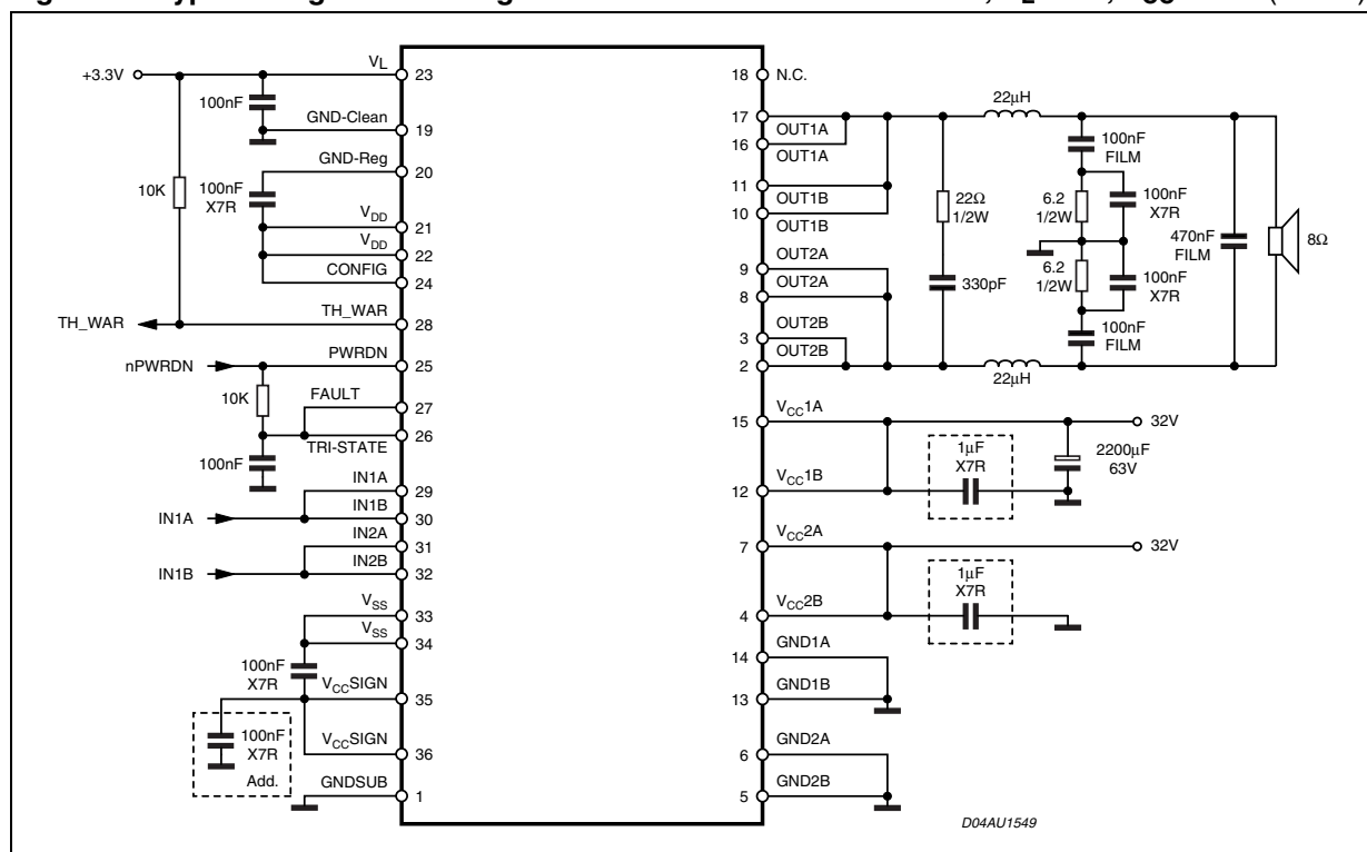
Figure 10. Typical Single BTL Configuration to Obtain 60W @ THD 10%, R_L = 8\Omega , V_{CC} = 32V (note 1)
