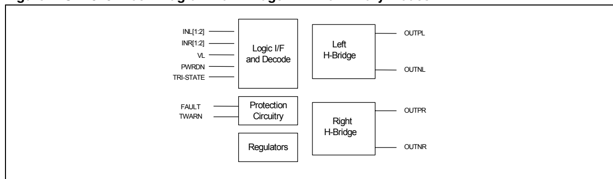
Figure 7. STA515 Block Diagram Full-Bridge DDX® or Binary Modes
