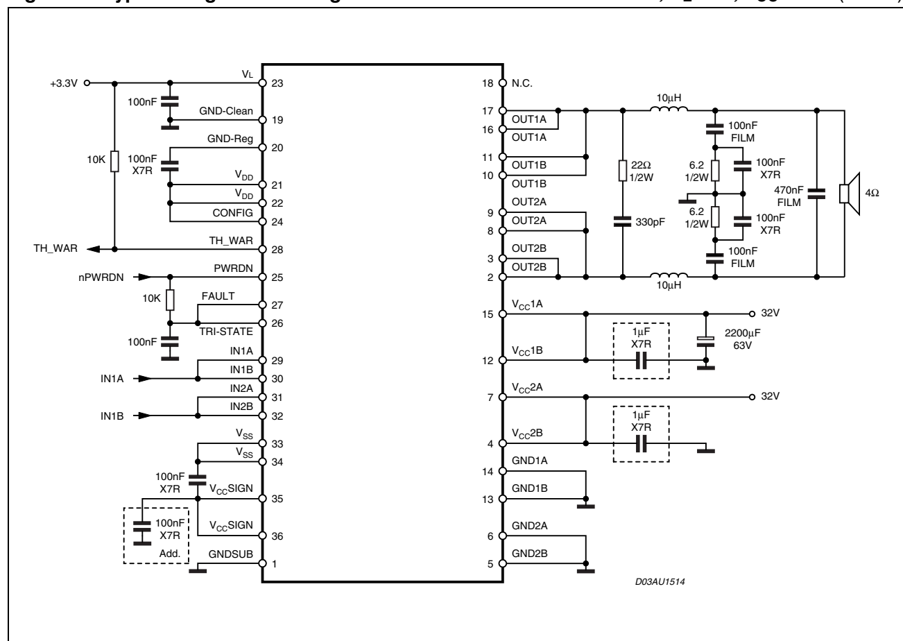
Figure 10. Typical Single BTL Configuration to Obtain 120W @ THD 10%, R_L = 4\Omega , V_{CC} = 32\text{V} (note 1))
