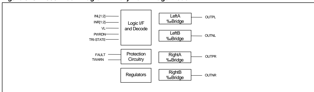
Figure 8. STA506 Block Diagram Binary Half-Bridge Mode
