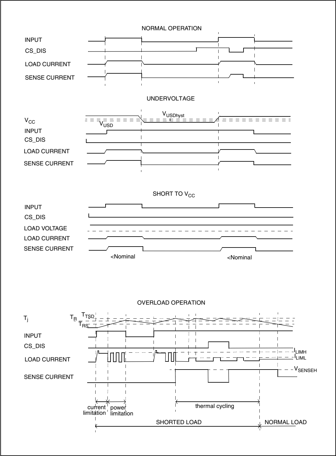
Figure 10. Waveforms
