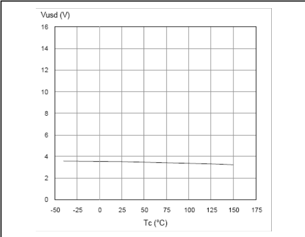
Figure 19. Undervoltage shutdown
