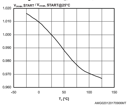
Figure 7: V_{DRAIN\_START} vs T_J
