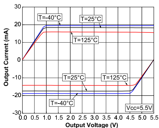
Figure 16: Output current vs. output voltage at VCC = 5.5 V
