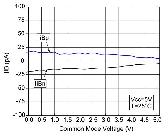
Figure 17: Input bias current vs. common mode at VCC = 5 V
