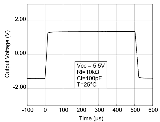
Figure 31: Large signal
