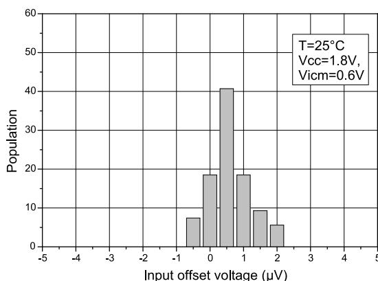
Figure 5: Input offset voltage distribution at VCC = 1.8 V
