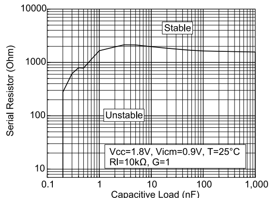
Figure 44: Stability criteria with a serial resistor at VDD = 1.8 V
