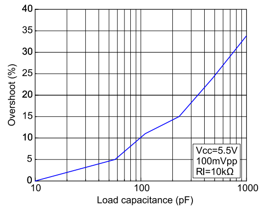
Figure 29: Output overshoot vs. load capacitance
