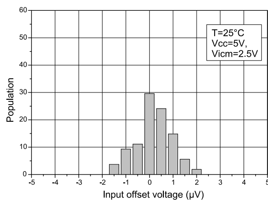
Figure 3: Input offset voltage distribution at VCC = 5 V
