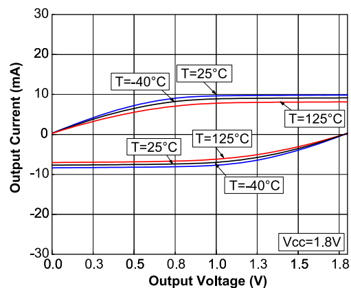
Figure 15: Output current vs. output voltage at VCC = 1.8 V
