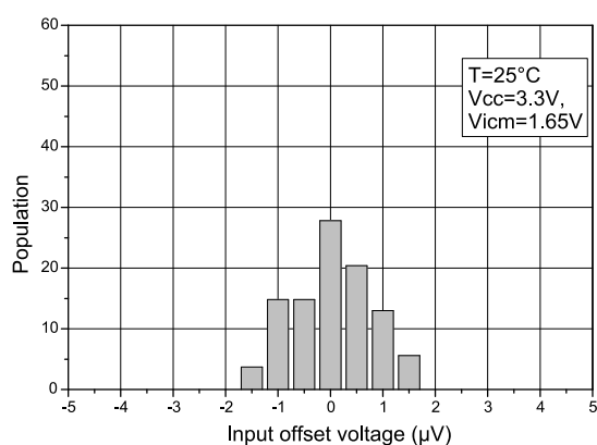
Figure 4: Input offset voltage distribution at VCC = 3.3 V
