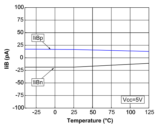
Figure 19: Input bias current vs. temperature at VCC = 5 V
