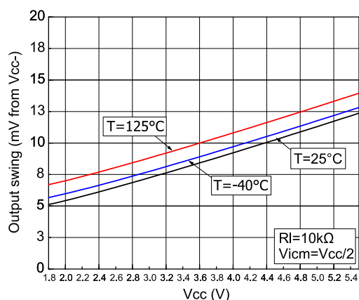
Figure 14: VOL vs. supply voltage
