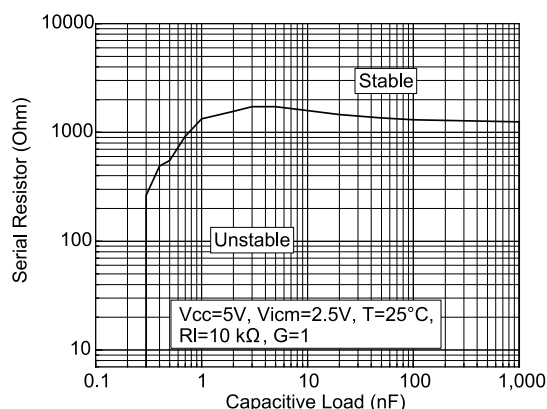
Figure 43: Stability criteria with a serial resistor at VDD = 5 V
