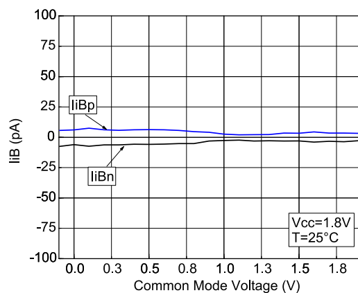
Figure 18: Input bias current vs. common mode at VCC = 1.8 V
