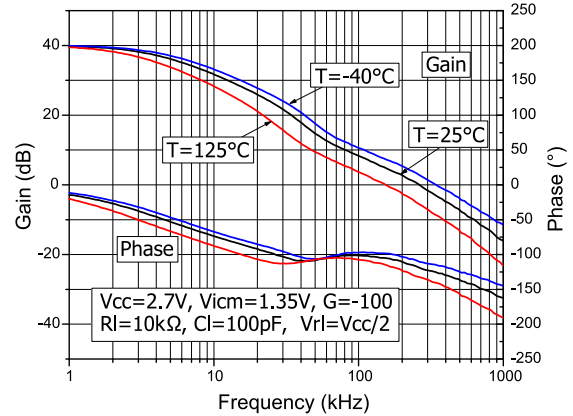
Figure 21: Bode diagram at VCC = 2.7 V
