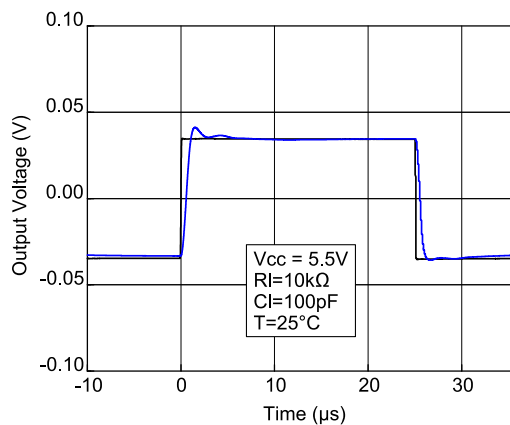
Figure 30: Small signal
