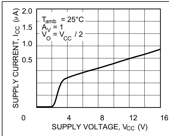
Figure 3. Supply current (each amplifier) vs. supply voltage
