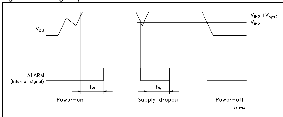
Figure 4. Voltage supervisor
