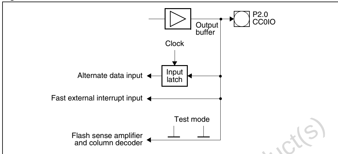
Figure 40. Port2 test mode structure
