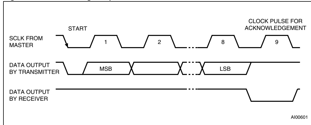
Figure 5. Acknowledge sequence
