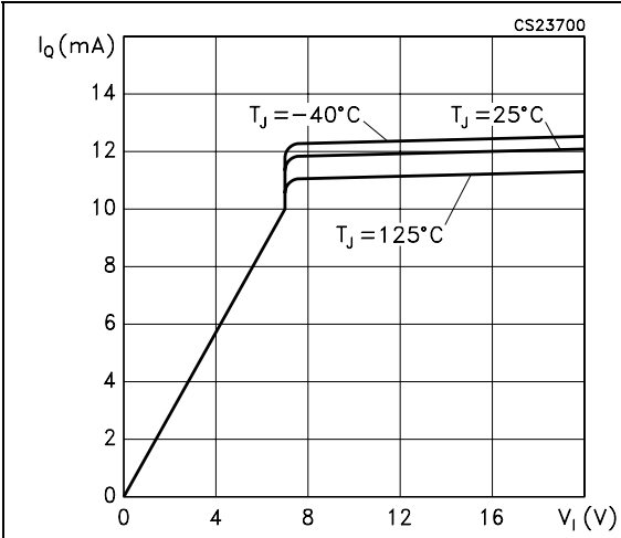
Figure 11. Quiescent current
