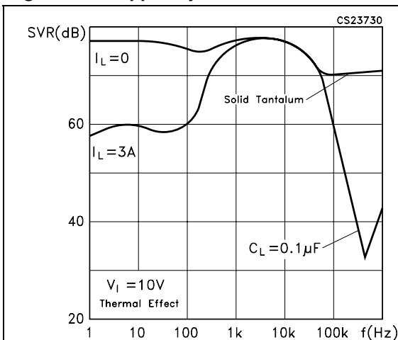
Figure 7. Ripple rejection
