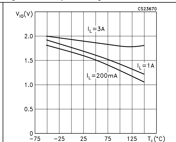
Figure 8. Dropout voltage
