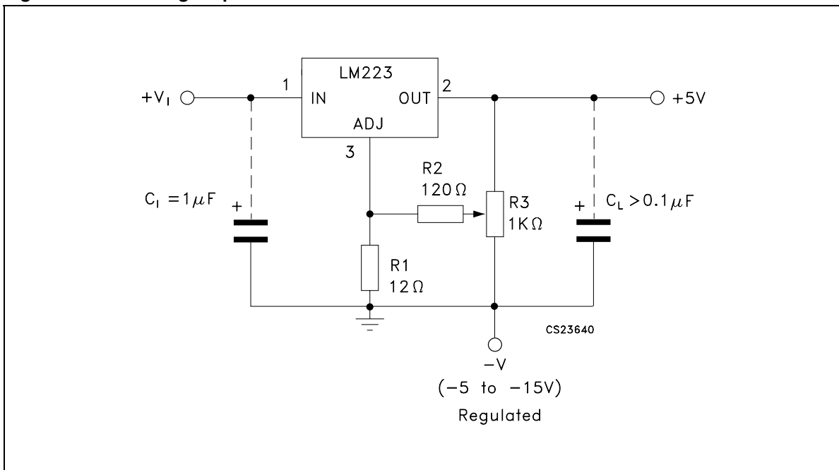
Figure 14. Trimming output to 5 V
