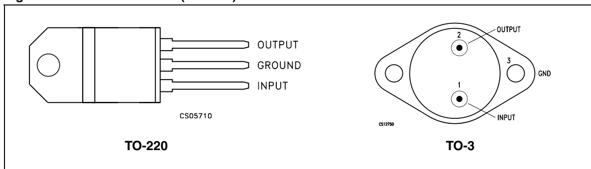
Figure 2. Pin connections (tot view)
