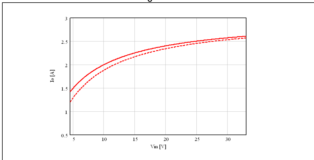
Figure 37. Maximum output current according to switch max. peak current (3.0 A): V_O = -5\text{ V}
