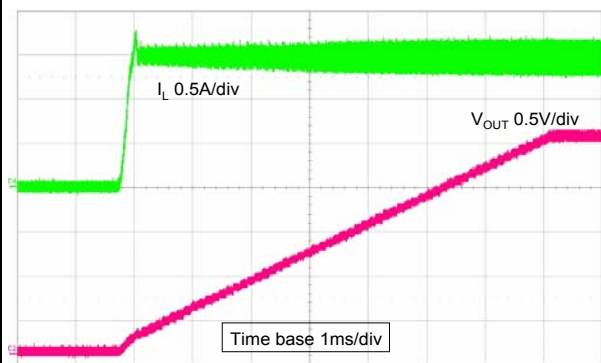
Figure 31. Soft-start
