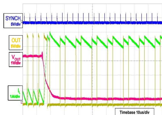
Figure 33. Short-circuit behavior V_{IN} = 24 V
