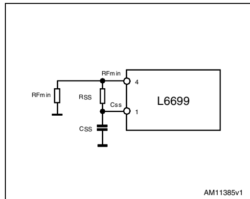
Figure 12. Soft-start circuit
