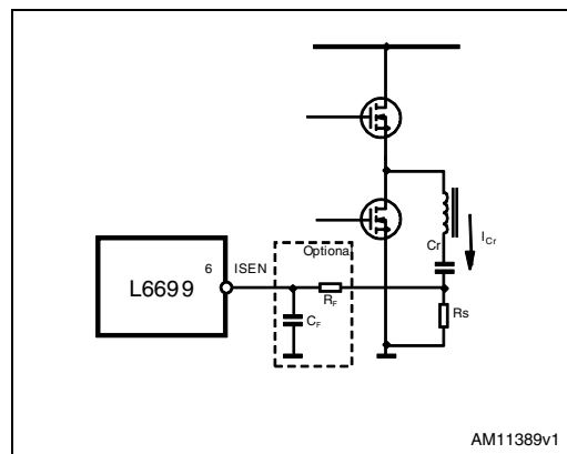
Figure 18. Current sensing techniques with sense resistor
