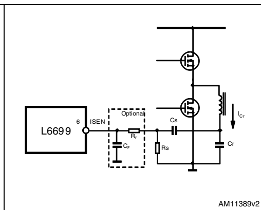
Figure 19. Current sensing techniques "lossless", with capacitive shunt
