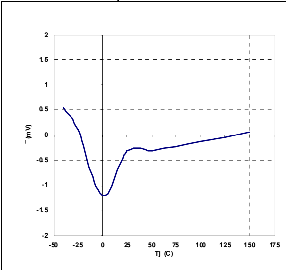
Figure 21. V_{MULTpk} - V_{VFF} dropout vs T_J
