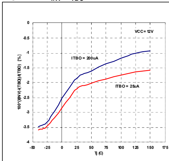
Figure 17. I_{INV} - I_{TBO} current mismatch vs T_J
