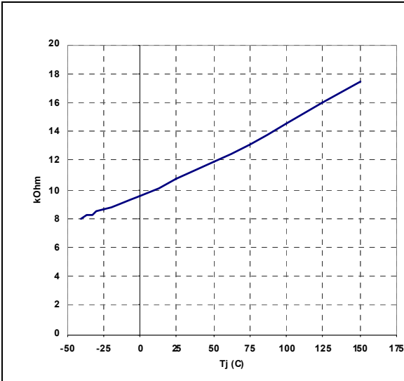
Figure 19. R discharge vs T_J
