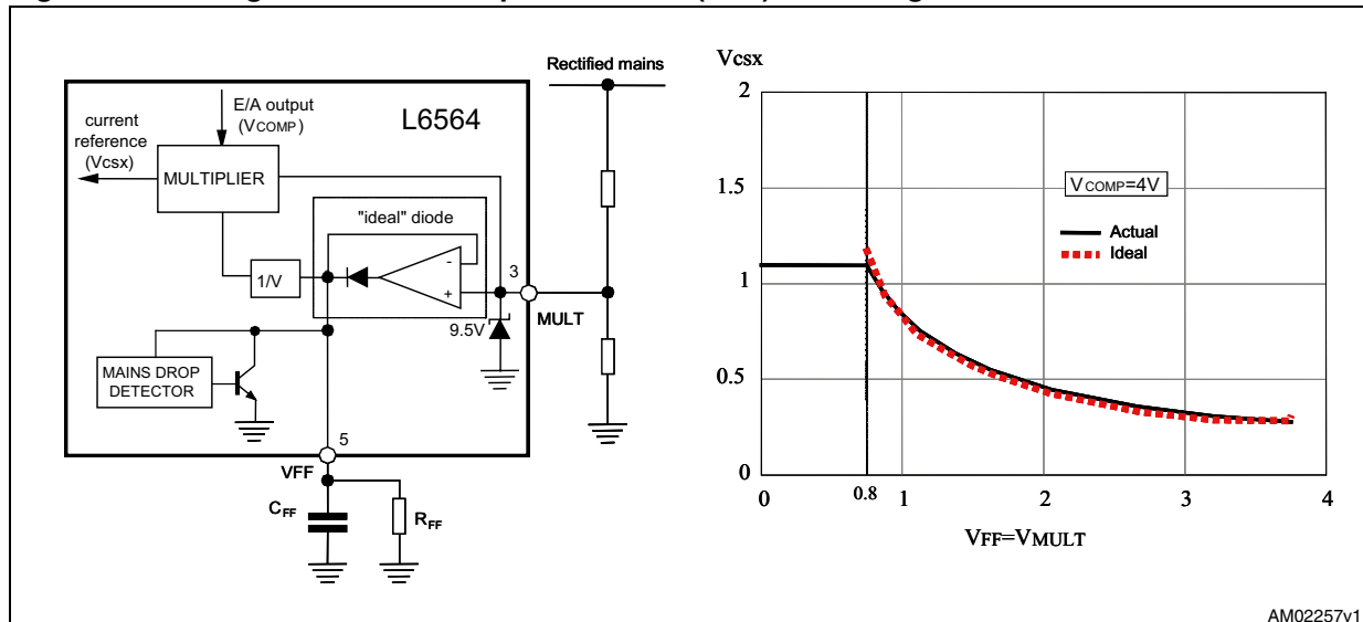
Figure 35. Voltage feedforward: squarer-divider ( 1/V^2 ) block diagram and transfer characteristic
