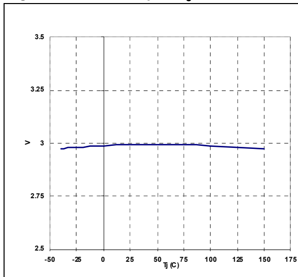
Figure 15. TBO clamp vs T_J
