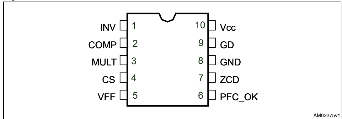
Figure 2. Pin connection
