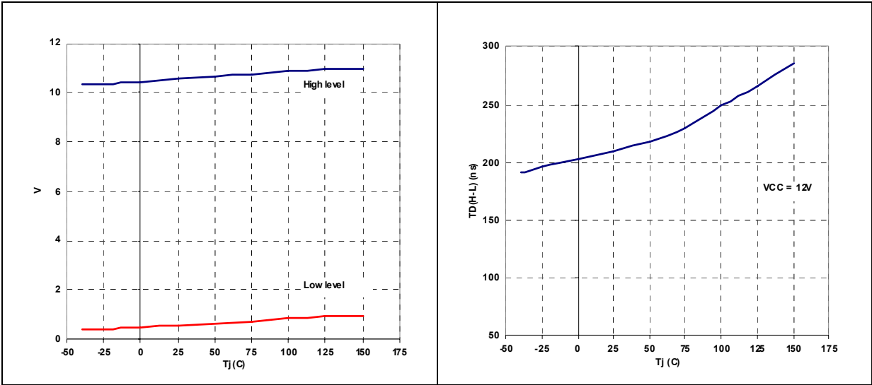
Figure 31. Gate drive output saturation vs T_J Figure 32. Delay to output vs T_J
