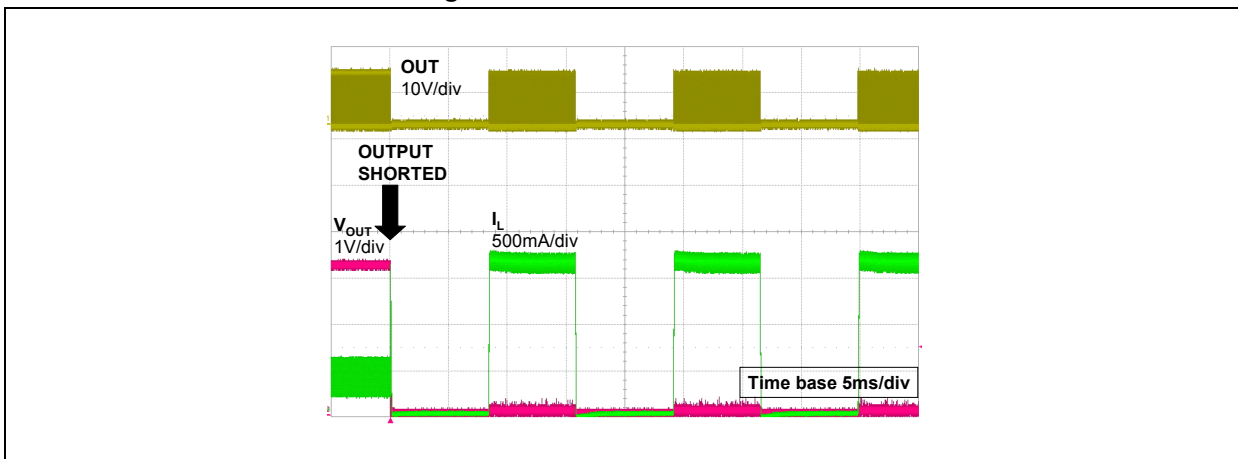
Figure 32. Short-circuit behavior
