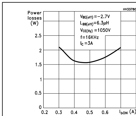
Figure 10. Power losses
