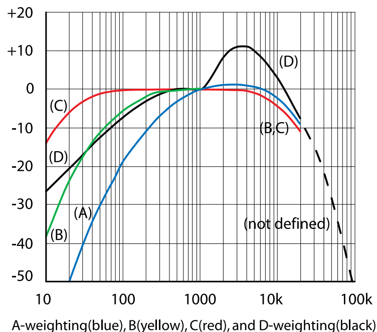
A-weighting curve
