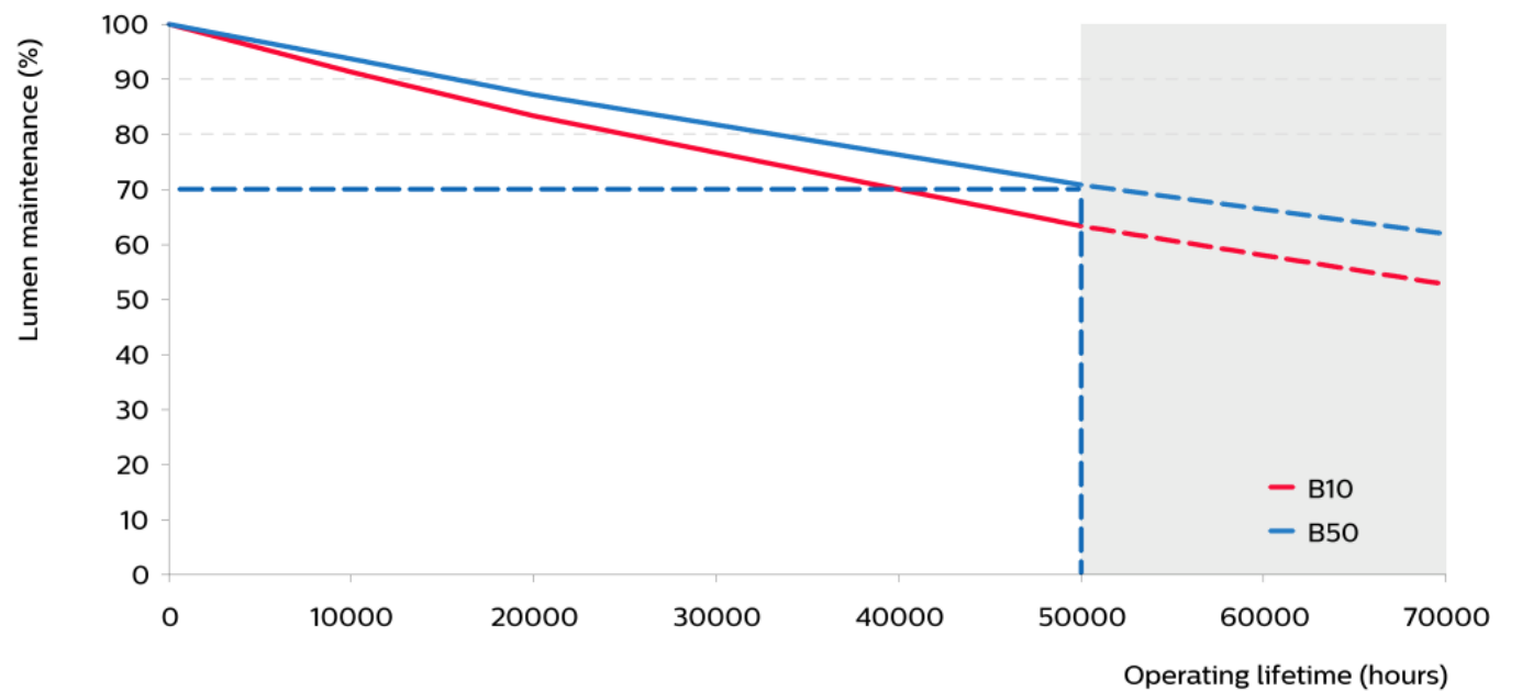
Lumen maintenance at I-life and Tc-life conditions
