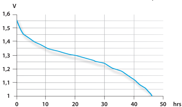
Remote Control: 15s/m 8h/d 24 ohm end 1,0 V
