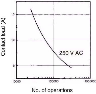
2. Life curve
