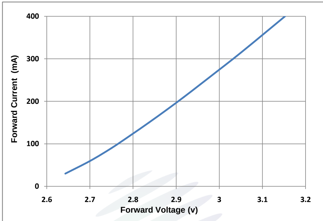
Fig 1-7 Forward Voltage Vs. Forward Current 伏安特性曲线 T_s=25^{\circ}\text{C}
