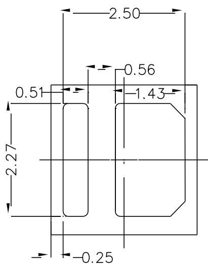
Fig.1-3 Bottom view
