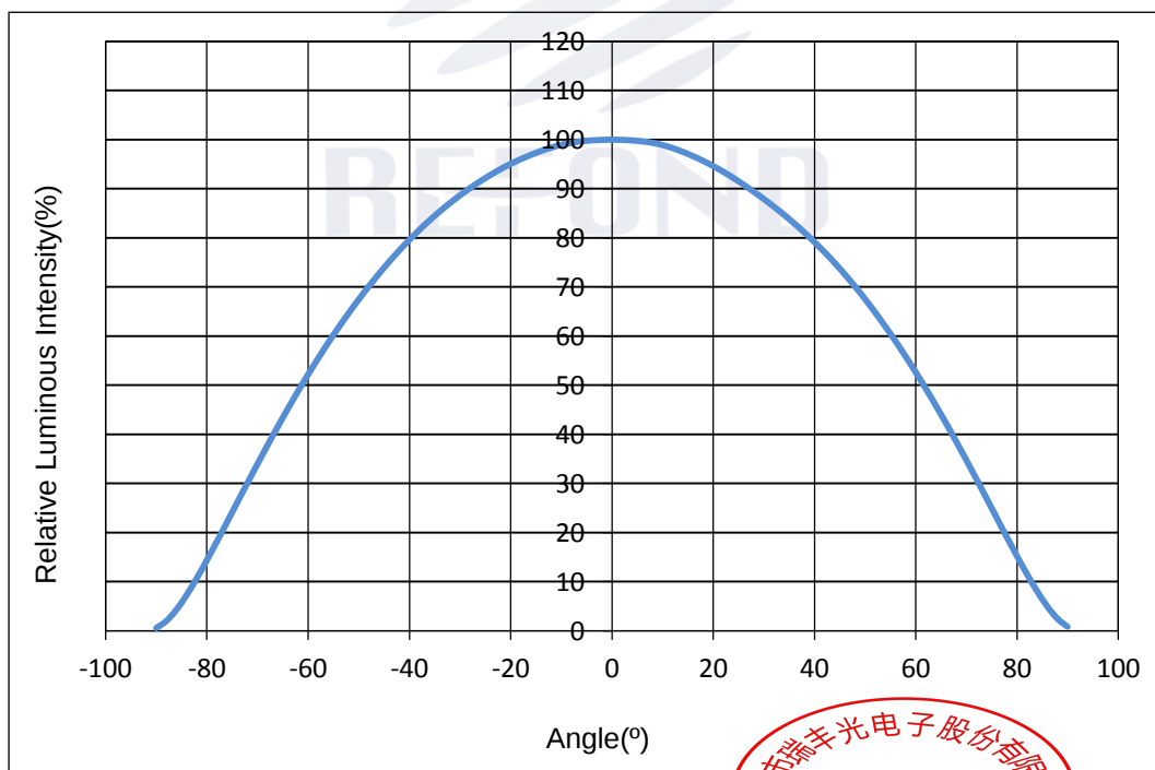
Fig 1-12 Radiation diagram
