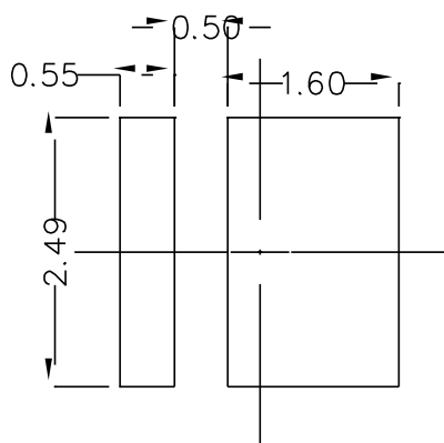
Fig.1-5 Soldering patterns
