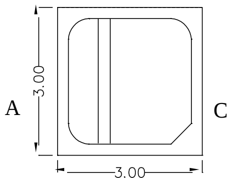
Fig.1-1 Top view
