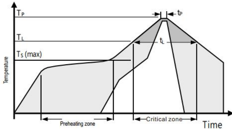
Figure 9. JEDEC Standard welding procedure diagram. T_P \leq 260^\circ\text{C} , t_P \leq 30 sec, lead-free welding. T_L \leq 220^\circ\text{C} , t_L \leq 150 sec, The rate of temperature rise and fall during welding shall be < 5^\circ\text{C}/\text{sec}
