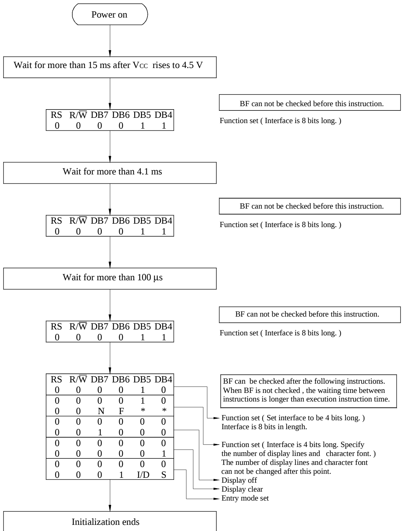
4-Bit Ineterface
