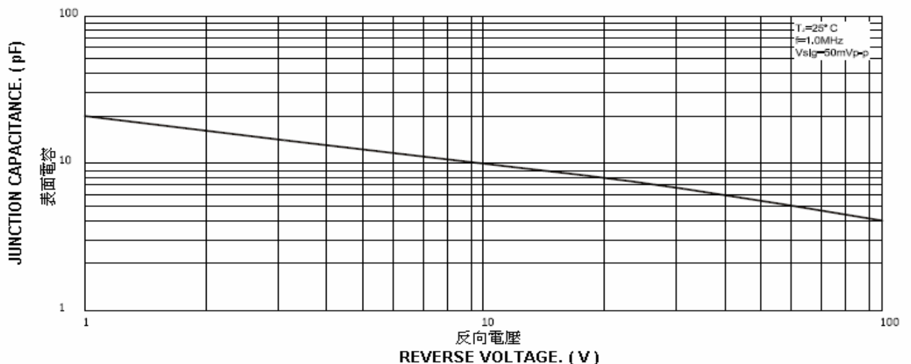
FIG. 5 –表面電容(典型值) FIG. 5 –TYPICAL JUNCTION CAPACITANCE
