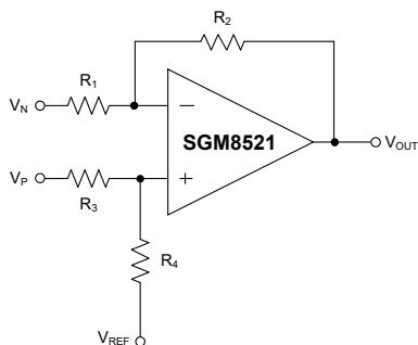
Figure 4. Differential Amplifier
