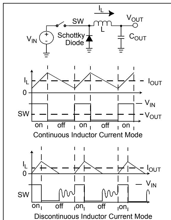
FIGURE 4-2: Step-Down Converter.
