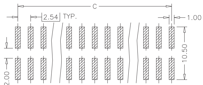
RECOMMEND P.C.B. LAYOUT TOP VIEW
