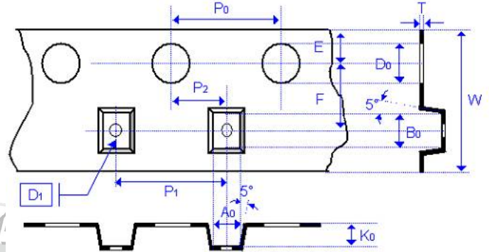
Fig. 9.2 The dimension of plastic tape
