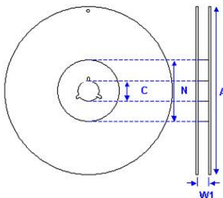
Fig. 9.3 The dimension of reel
