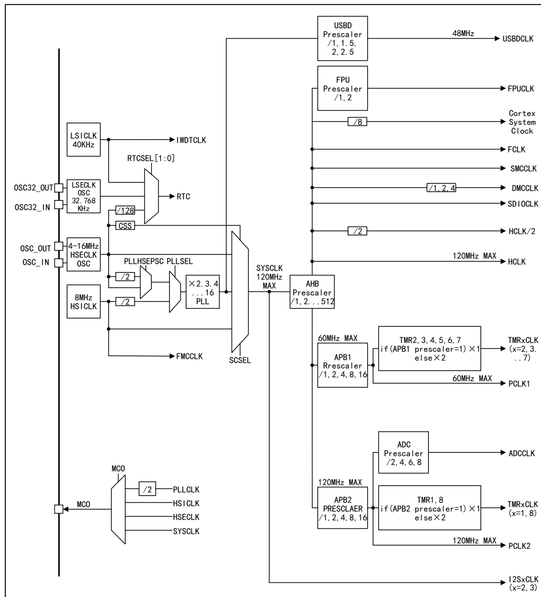
Figure 8 APM32E103xCxE Clock Tree
