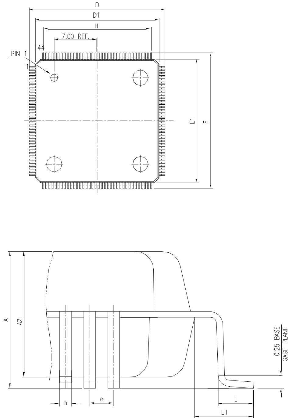
Figure 18 LQFP144 Package Diagram
