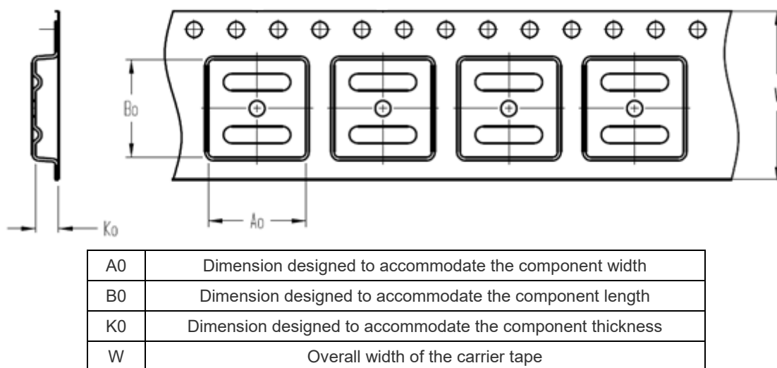
Figure 33 Specification Drawing of Reel Packaging
