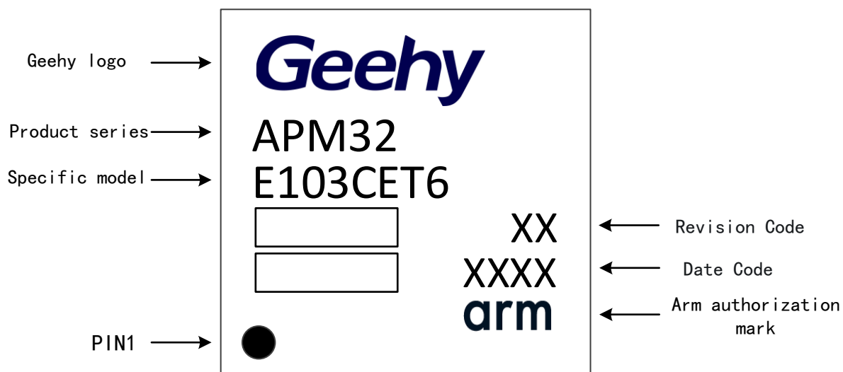
Figure 29 LQFP48-48 pins, 7×7mm identification diagram
